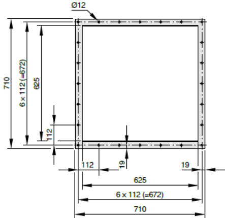
KSF, flange dimensions for filter 610 × 610
