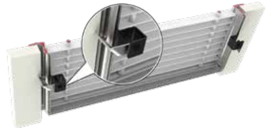
Concealed screw fixings without installation subframe
